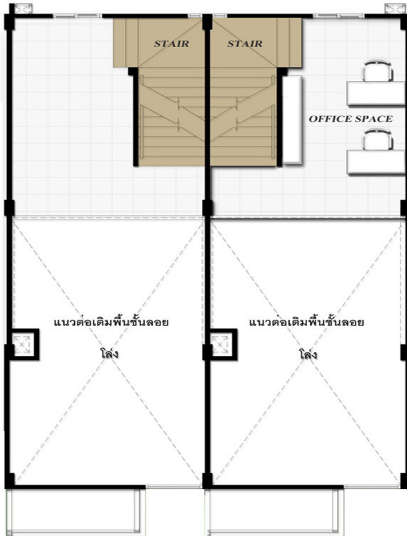
BUILDING C-D FLOOR PLAN
