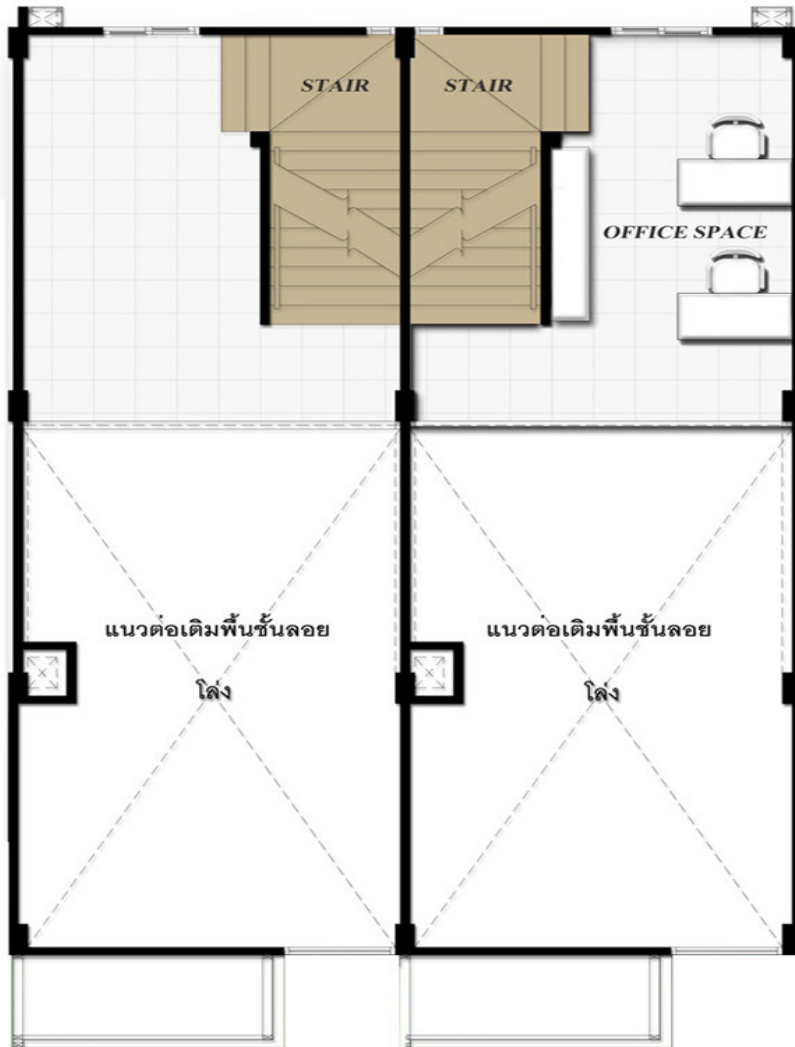
BUILDING A-B FLOOR PLAN
